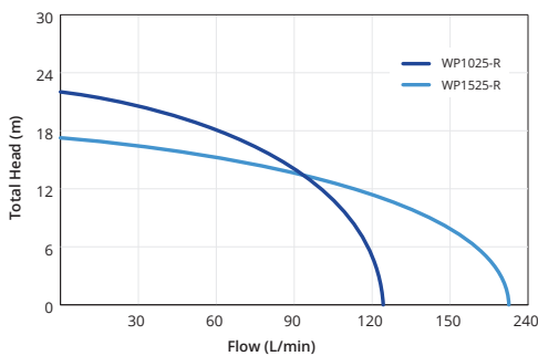
Performance Curve
