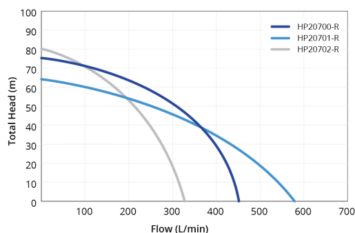
Performance Curve
