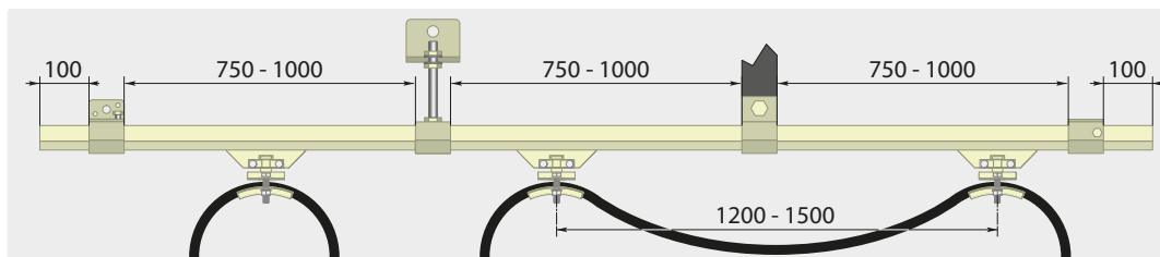
U-rails
