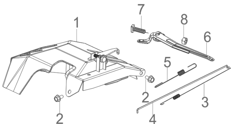
FIG.11 CONTROL ASSY, THROTTLE (E11)
