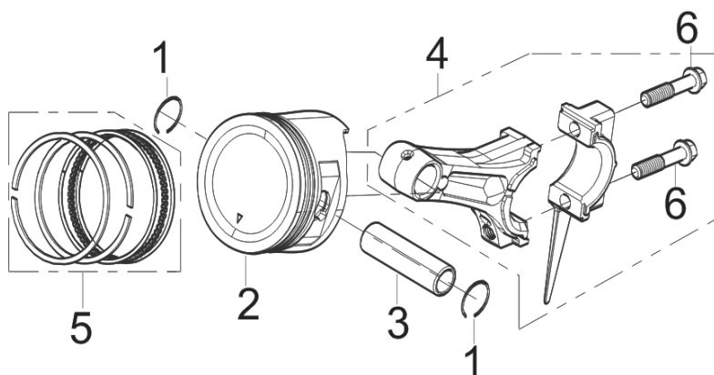
FIG.5 RING SET,OIL / ROD,CRANKSHAFT CONNETING (E05)
