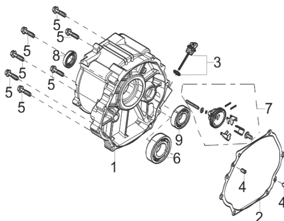
FIG.2 COVER SUBASSEMBLY, CRANKCASE (E02)
