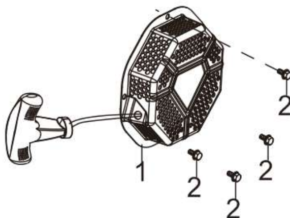
FIG.7 STARTER,RECOIL (E07)
