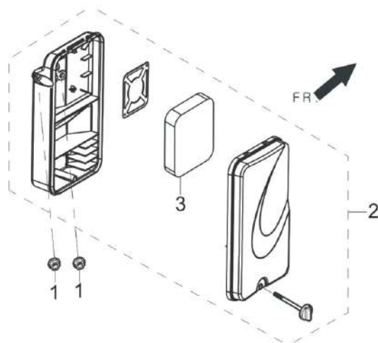
FIG.13 CLEANER, AIR (F01)
