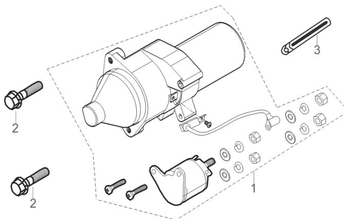
FIG.12 MOTOR ASSY, STARTING (E12)
