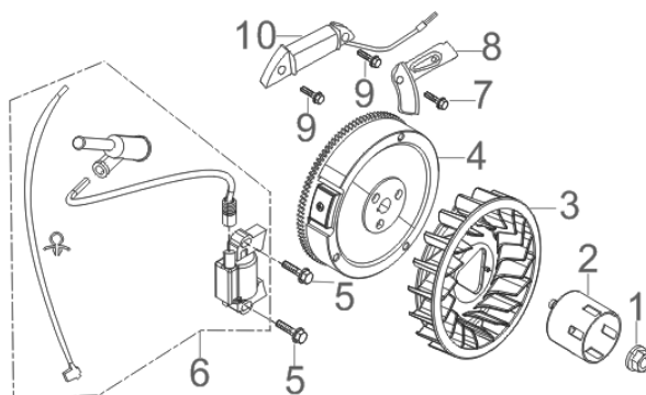
FIG.10 FLYWHEEL / IMPELLER / STARTER PULLEY / IGNITION COIL (E10)
