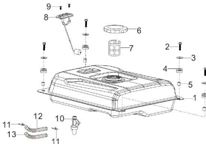
FIG.15 TANK ASSY, FUEL (F03)
