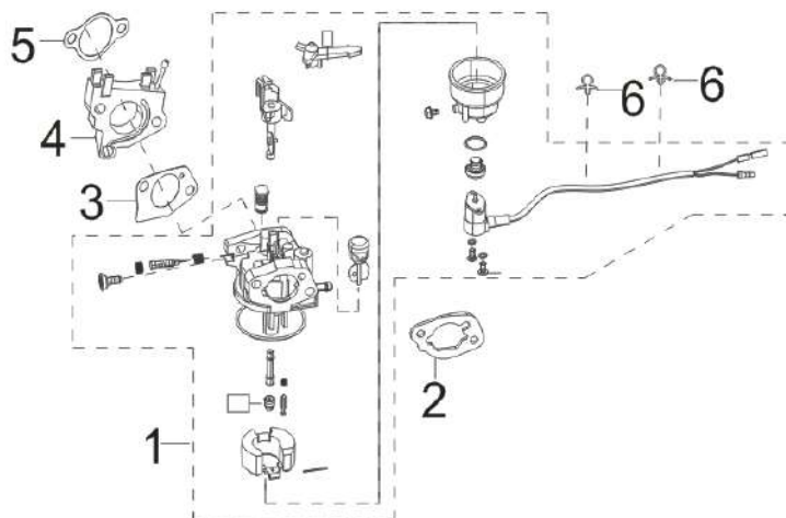
FIG.9 CARBURETOR ASSY. (E09)
