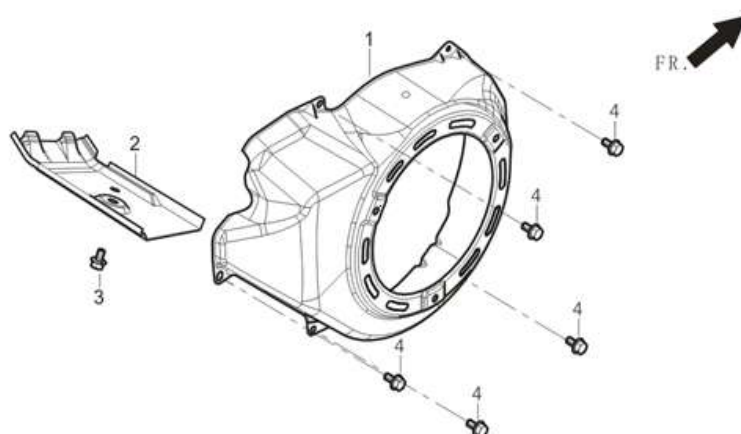
FIG.8 SHROUD / SHIELD,LOWER (E08)
