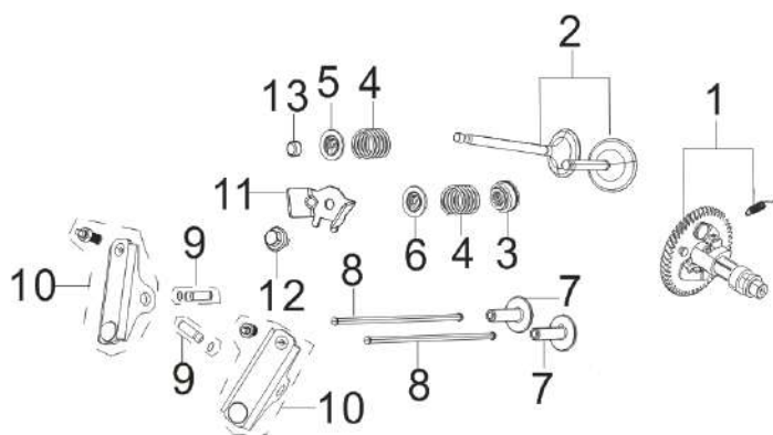
FIG.6 TRAIN,VALVE / CAMSHAFT SUBASSEMBLY (E06)
