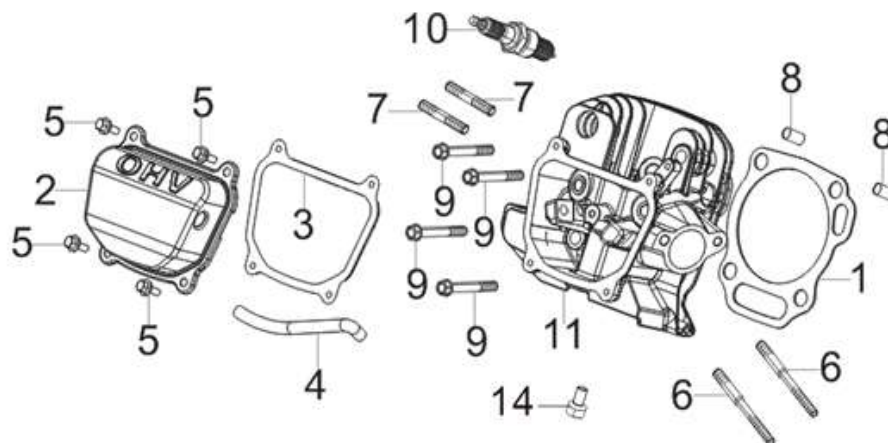
FIG.3 HEAD SUBASSEMBLY, CYLINDER / PLUG, SPARK (E03)
