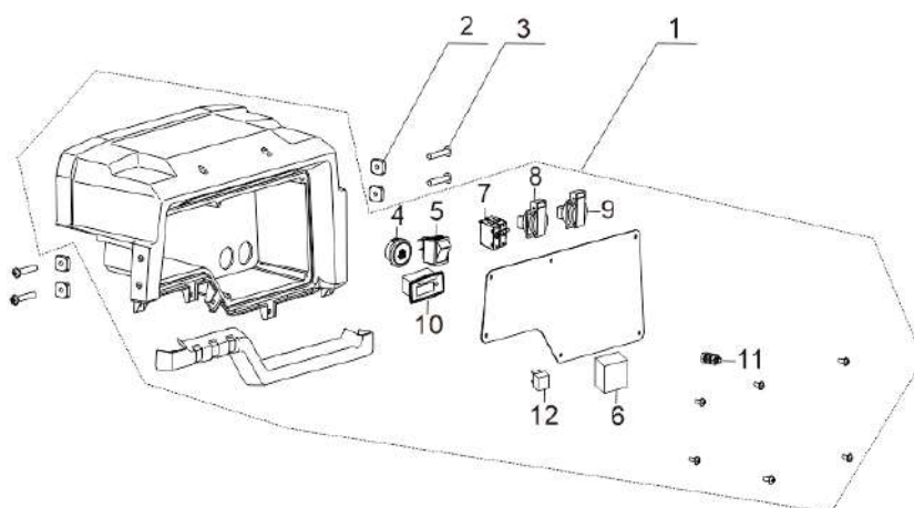
FIG.17 PANEL SUBASSEMBLY, CONTROL (F05)
