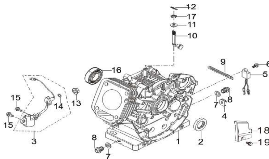
FIG.1 CRANKCASE. / GEAR ASSY, GOVERNOR. (E01)
