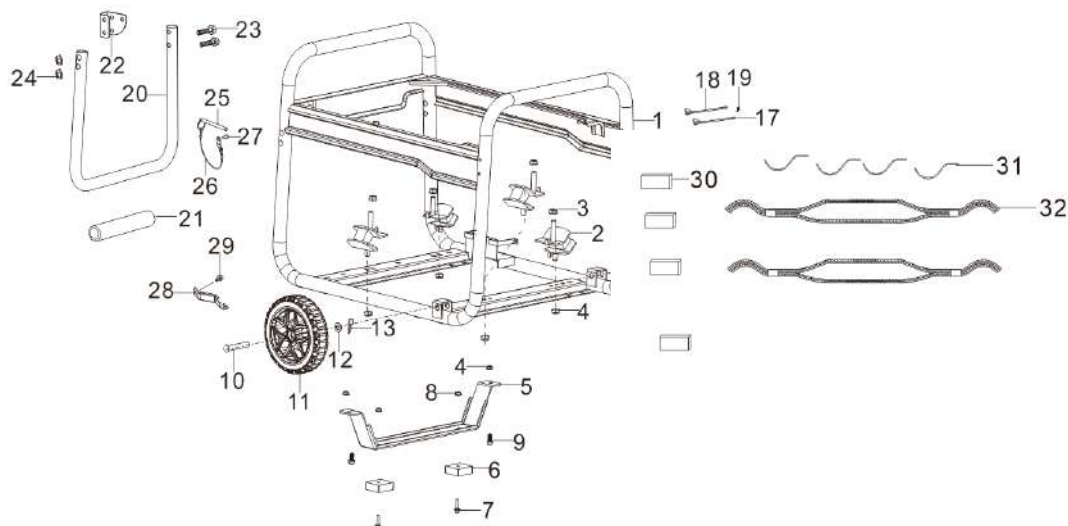
FIG.16 FRAME, ENGINE ( F04 )
