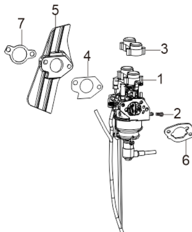
FIG.8 CARBURETOR ASSY. (E09)
