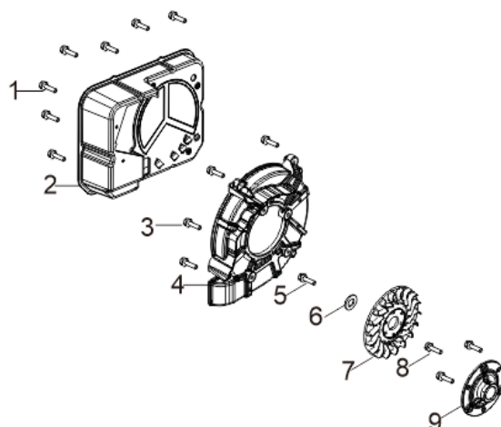
FIG.12 MUFFLER ASSY. (F03)
