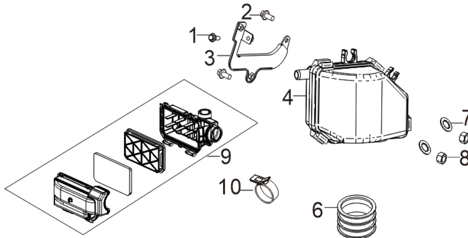
FIG.10 AIR CLEANER (F01)
