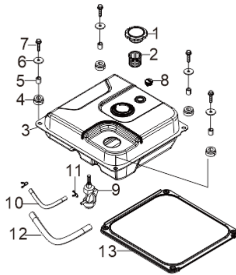
FIG.14 TANK ASSY, FUEL (F05)
