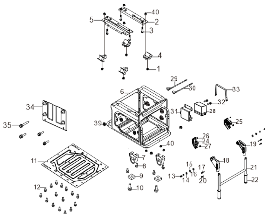
FIG.15 FRAME, ENGINE ( F06 )
