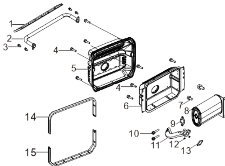
FIG.11 MUFFLER ASSY. (F02)
