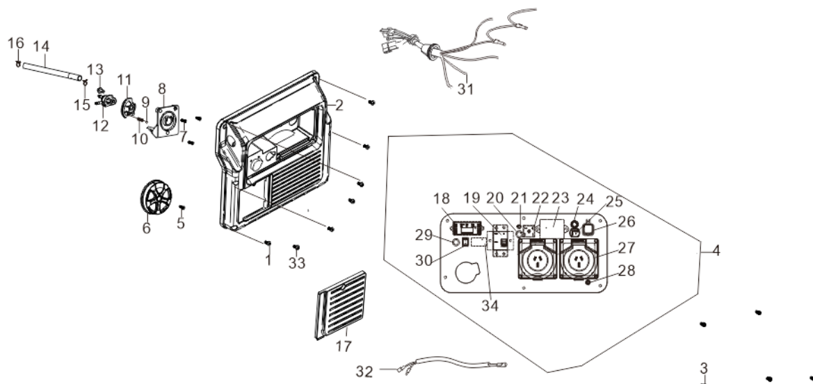
FIG.16 PANEL SUBASSEMBLY, CONTROL ( F07 )
