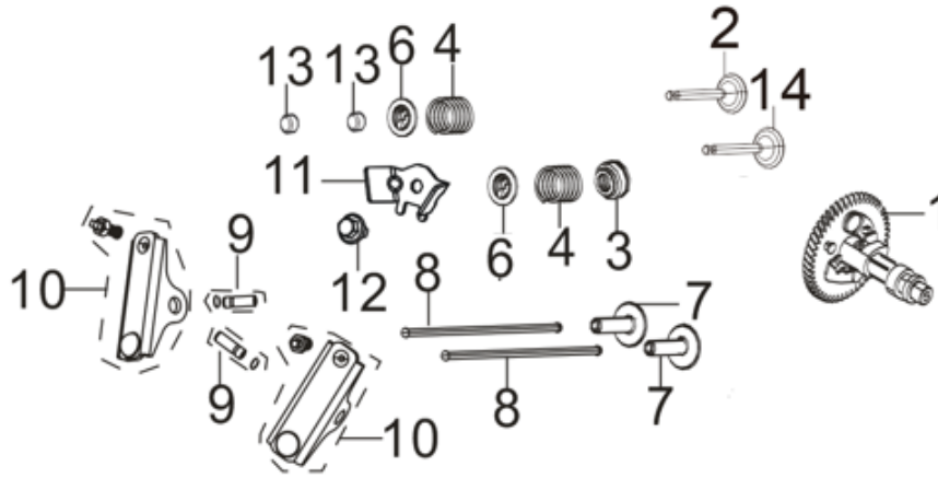
FIG.6 TRAIN,VALVE / CAMSHAFT SUBASSEMBLY (E06)
