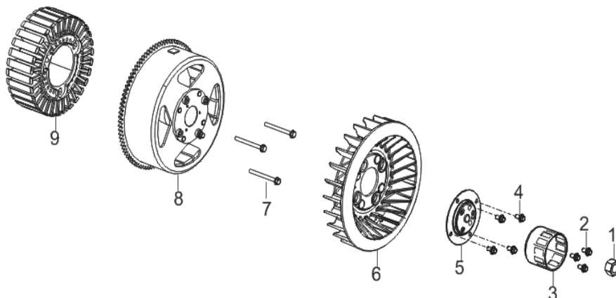
FIG.9 FLYWHEEL / IMPELLER / STARTER PULLEY / IGNITION COIL (E10)
