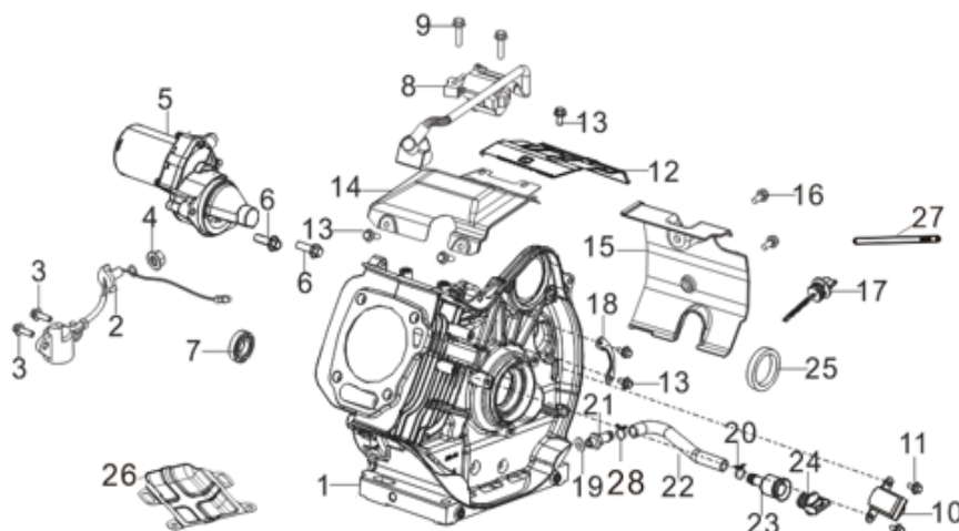
FIG.1 CRANKCASE. / GEAR ASSY, GOVERNOR. (E01)
