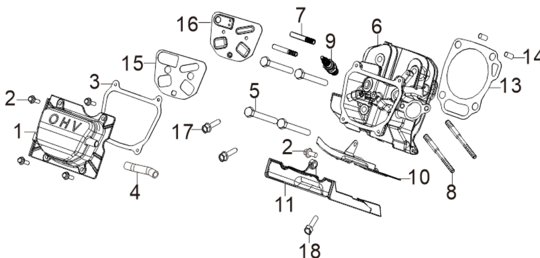
FIG.3 HEAD SUBASSEMBLY, CYLINDER / PLUG, SPARK (E03)
