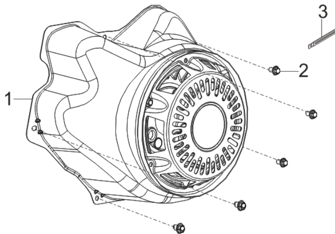
FIG.7 STARTER,RECOIL (E07)
